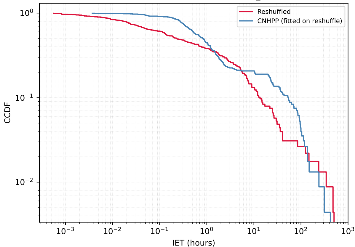
User 5689570195 - Reshuffled vs CNHPP A_{\text{fit}}=1.1787
