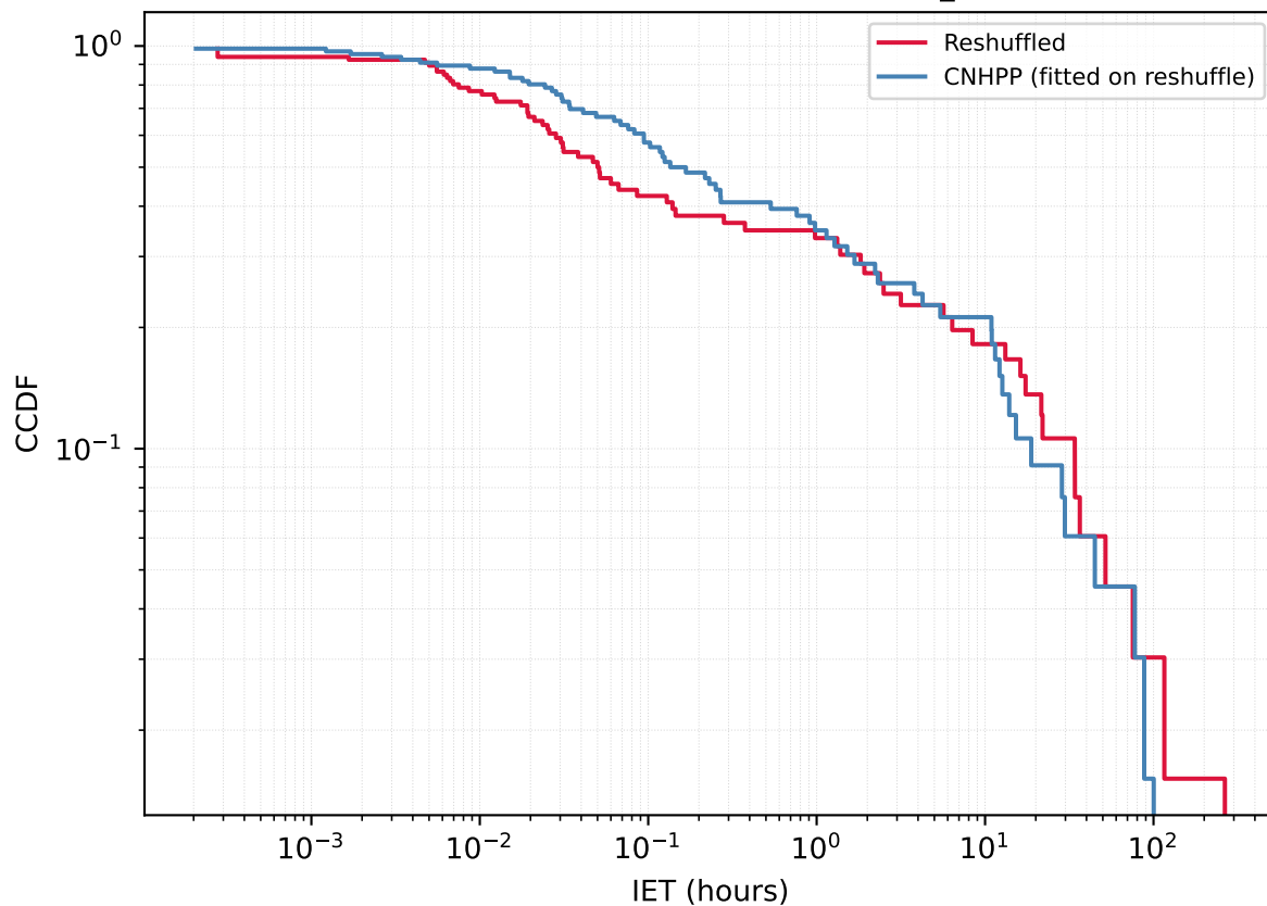
User 1527488629 - Reshuffled vs CNHPP A_{\text{fit}}=1.2824
