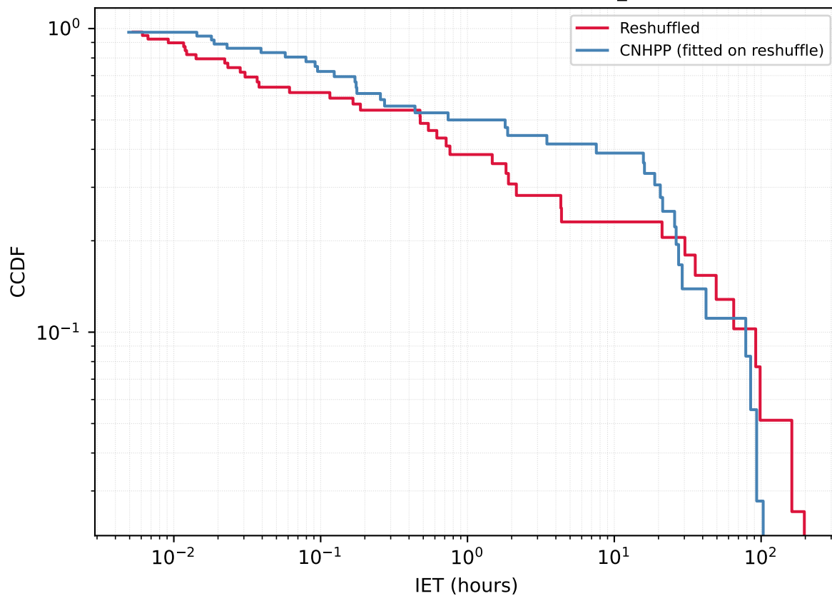
User 7286408806 - Reshuffled vs CNHPP A_{\text{fit}}=0.9278
