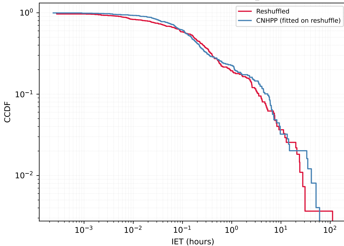
User 6221273187 - Reshuffled vs CNHPP A_{\text{fit}}=0.6332
