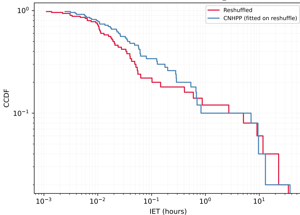
User 1383986630 - Reshuffled vs CNHPP A_{\text{fit}}=0.6629
