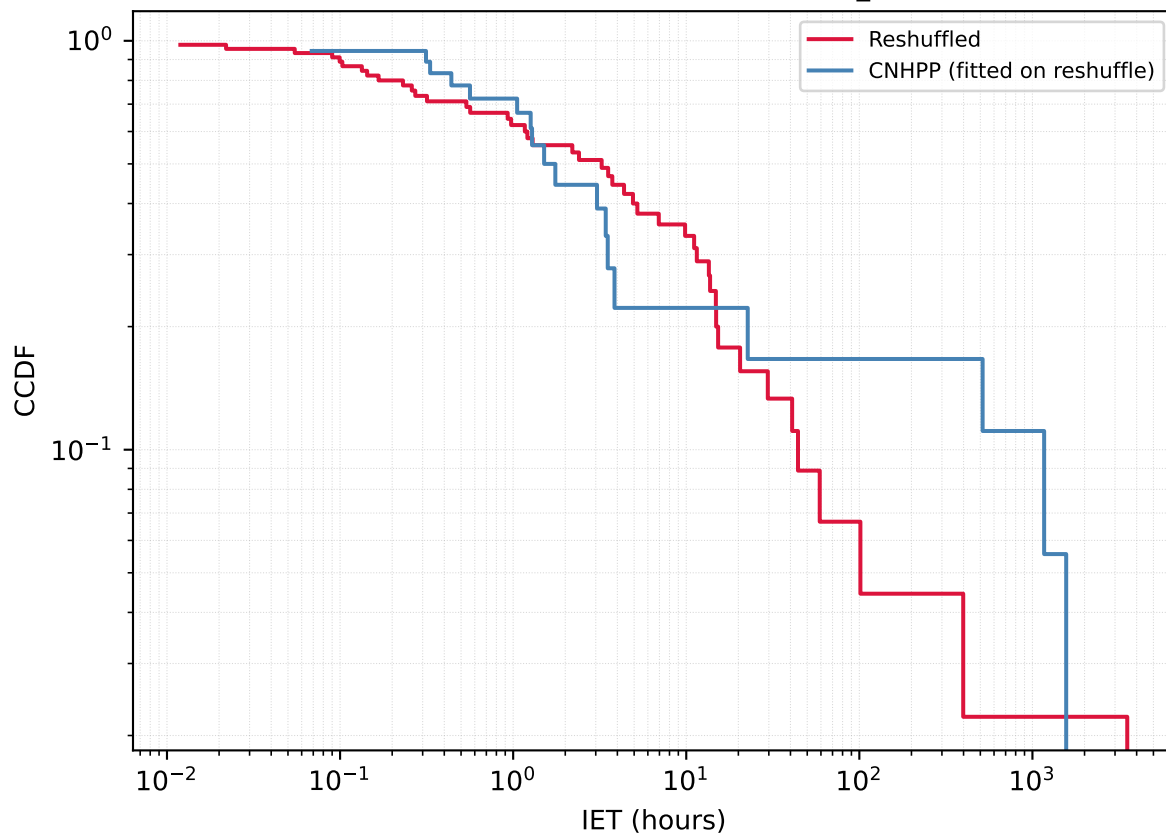
User 373434202 - Reshuffled vs CNHPP A_{\text{fit}}=1.3787
