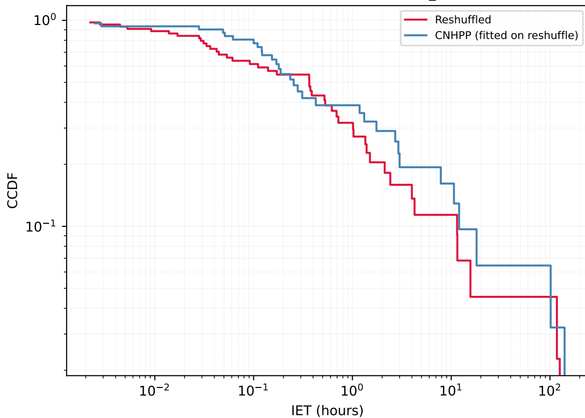
User 709835653 - Reshuffled vs CNHPP A_{\text{fit}}=0.7630
