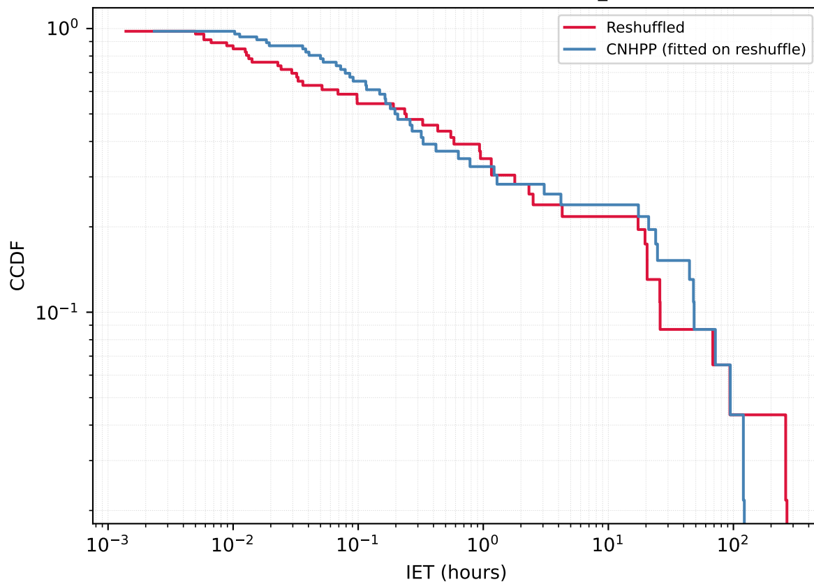
User 650840442 - Reshuffled vs CNHPP A_{\text{fit}}=0.8094
