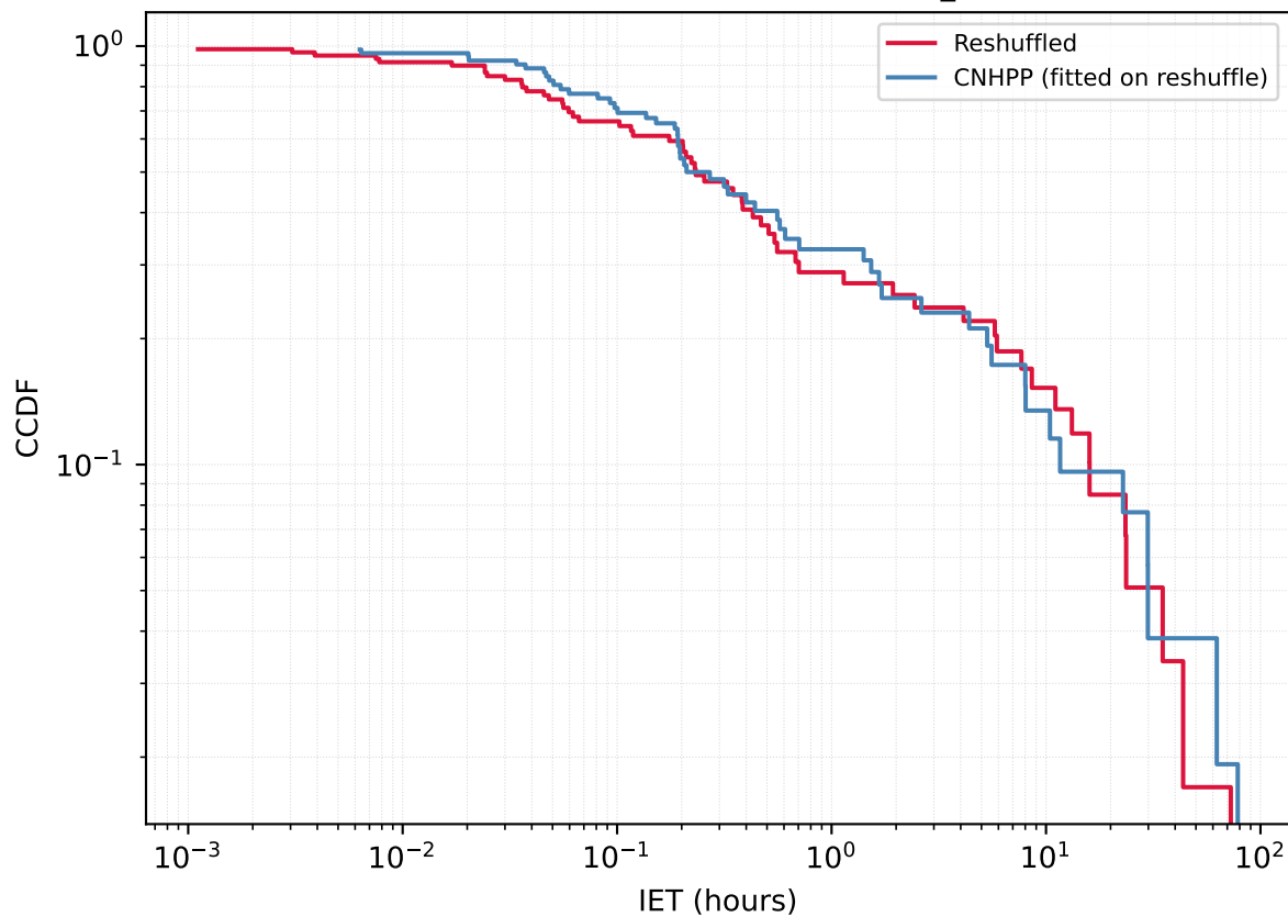
User 852631182 - Reshuffled vs CNHPP A_{\text{fit}}=0.4056
