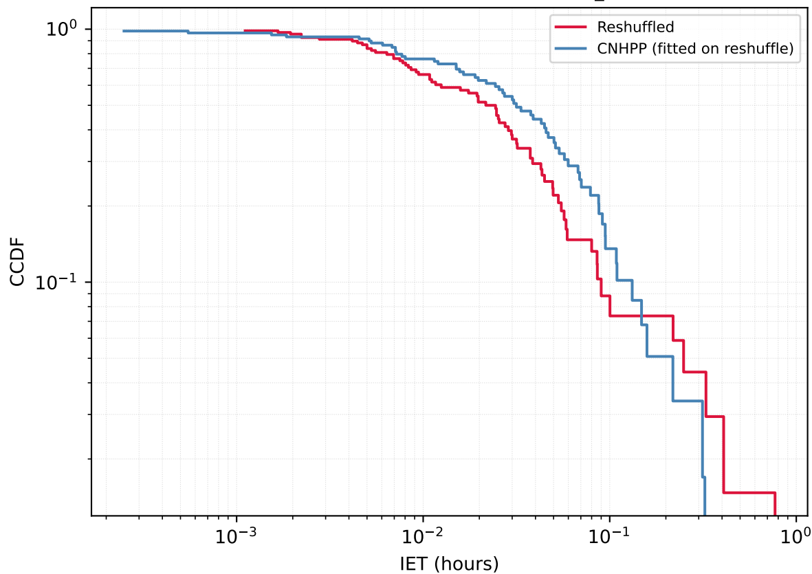
User 1179144696 - Reshuffled vs CNHPP A_{\text{fit}}=0.3128
