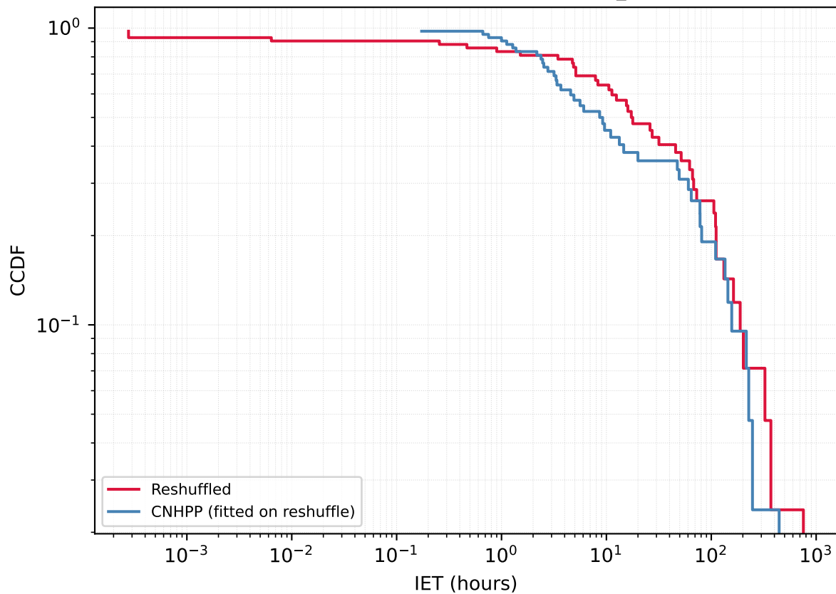
User 1154304070 - Reshuffled vs CNHPP A_{\text{fit}}=0.6064
