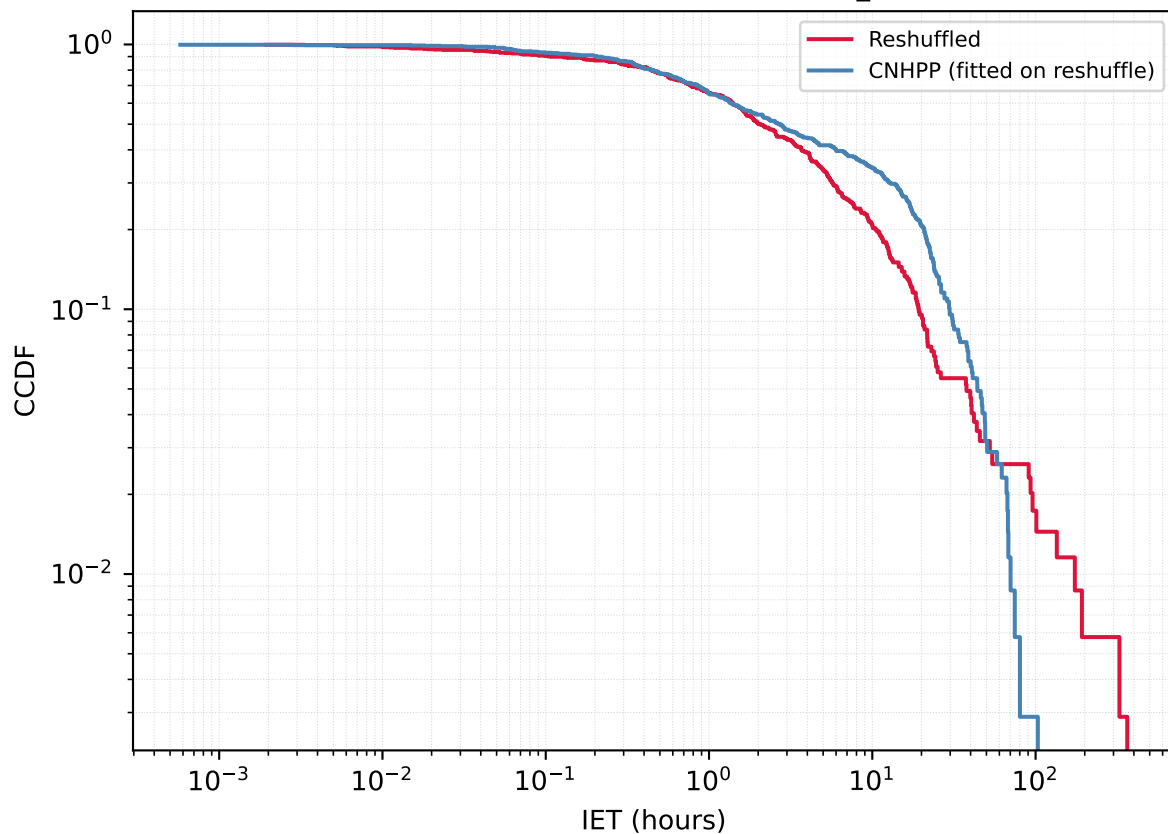
User 271855505 - Reshuffled vs CNHPP A_{\text{fit}}=0.3834
