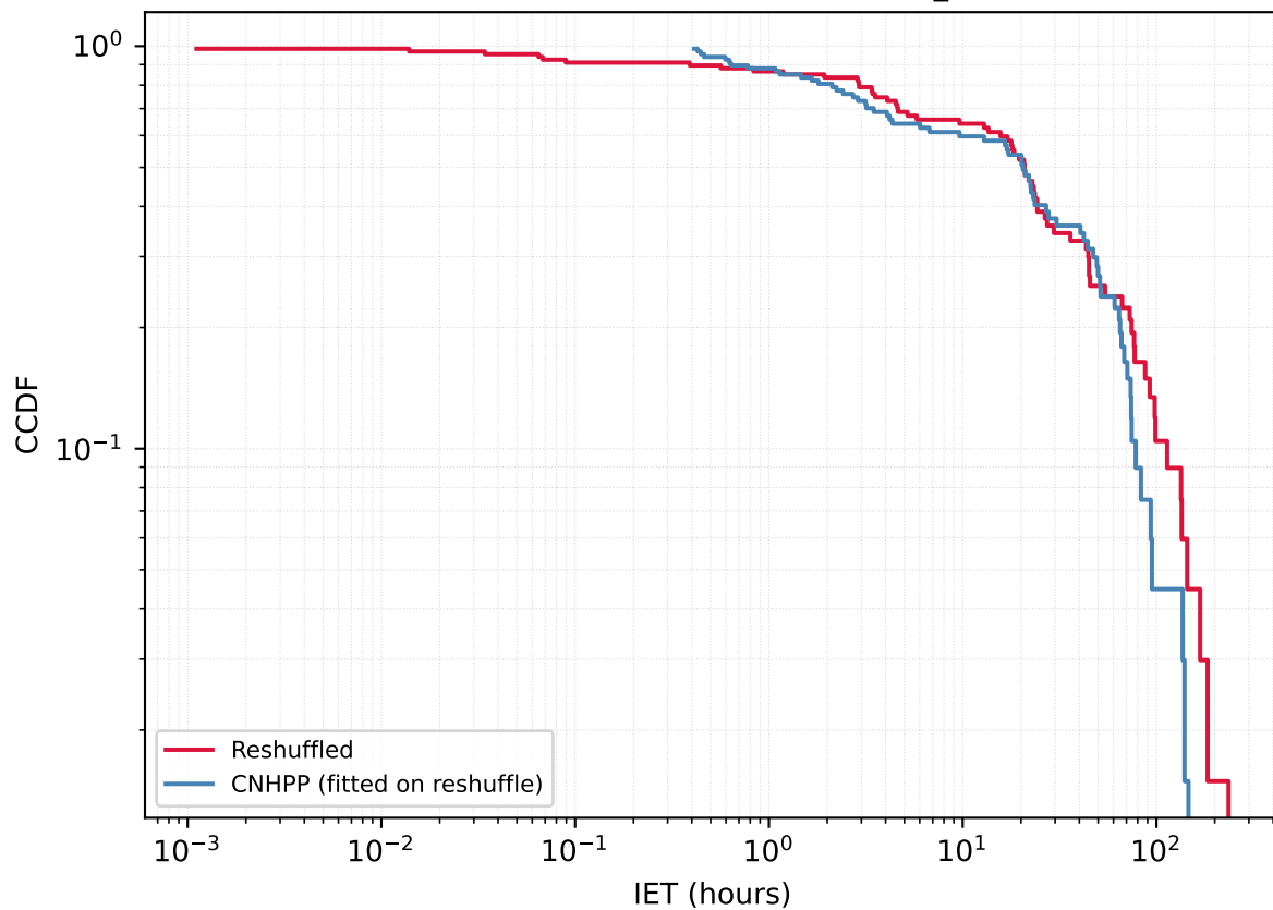
User 179738679 - Reshuffled vs CNHPP A_{\text{fit}}=0.2723
