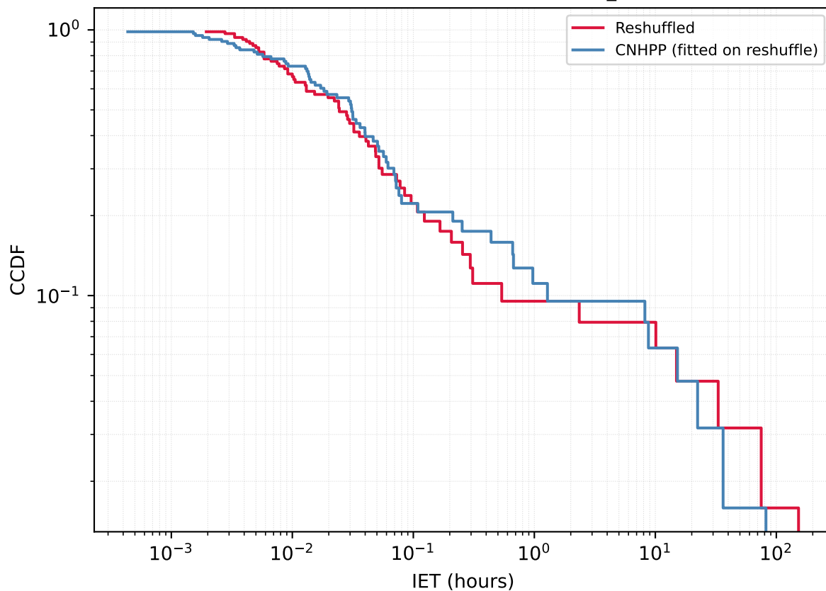
User 468916394 - Reshuffled vs CNHPP A_{\text{fit}}=0.3424
