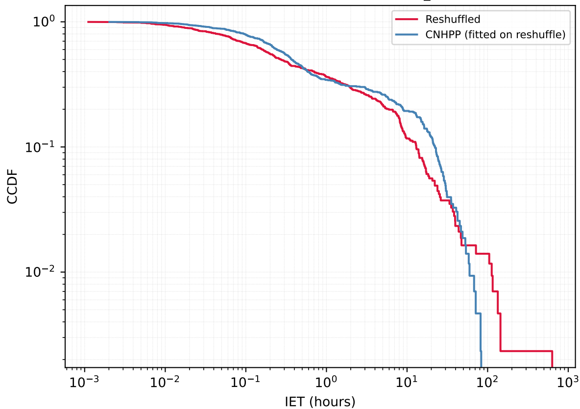
User 7094531229 - Reshuffled vs CNHPP A_{\text{fit}}=0.5353
