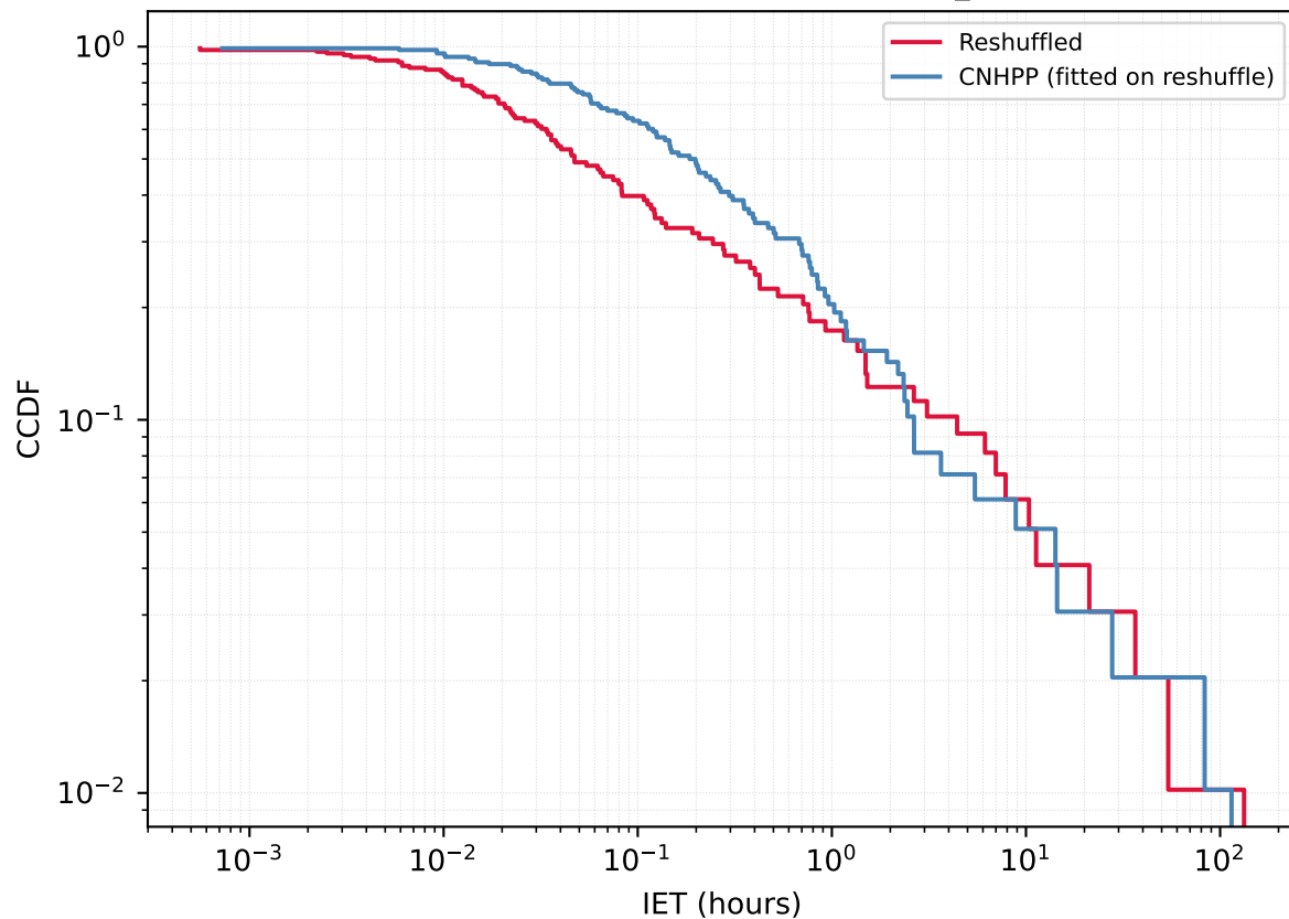
User 5564321416 - Reshuffled vs CNHPP A_fit=1.1597
