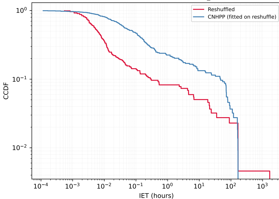
User 1457424889 - Reshuffled vs CNHPP A_{\text{fit}}=1.9228
